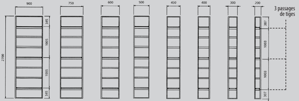
Panneaux H = 2700 mm
